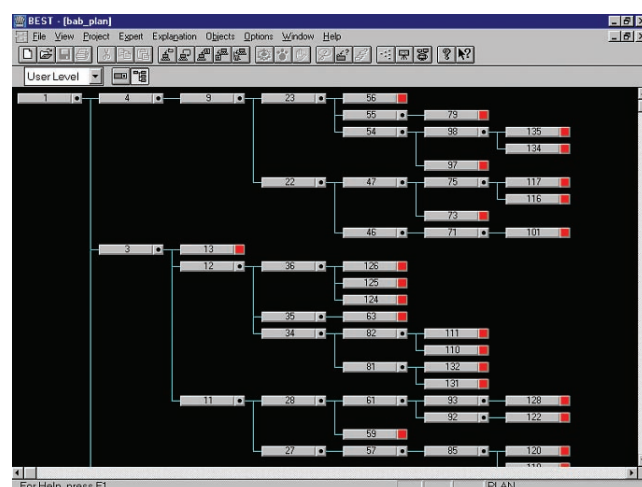
A decision tree for the branch-and-bound search strategy
