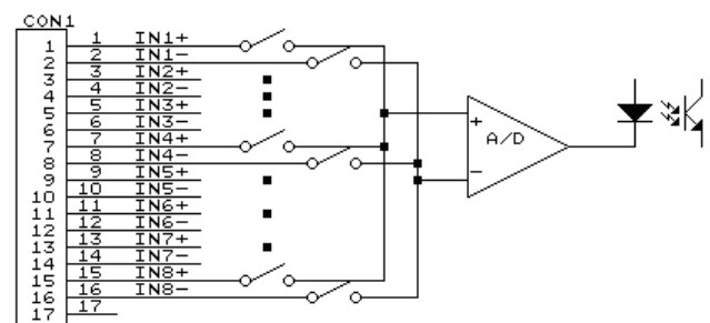
INPUT CIRCUIT DIAGRAM:
